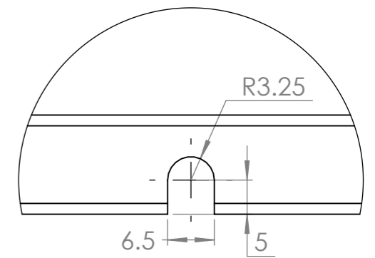
DETAIL A SCALE 2 : 1.5
